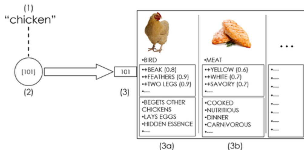
Figure 4: Yet another example of the same label that could point to separate arrays of information stored at the lower level. Chicken-qua-bird is stored at a different memory address than chicken-qua-meat, even though they are served by the same concept, 'chicken.' Chicken is thus a generative pointer insofar as it could generate one or another, contingent on the task at hand.
