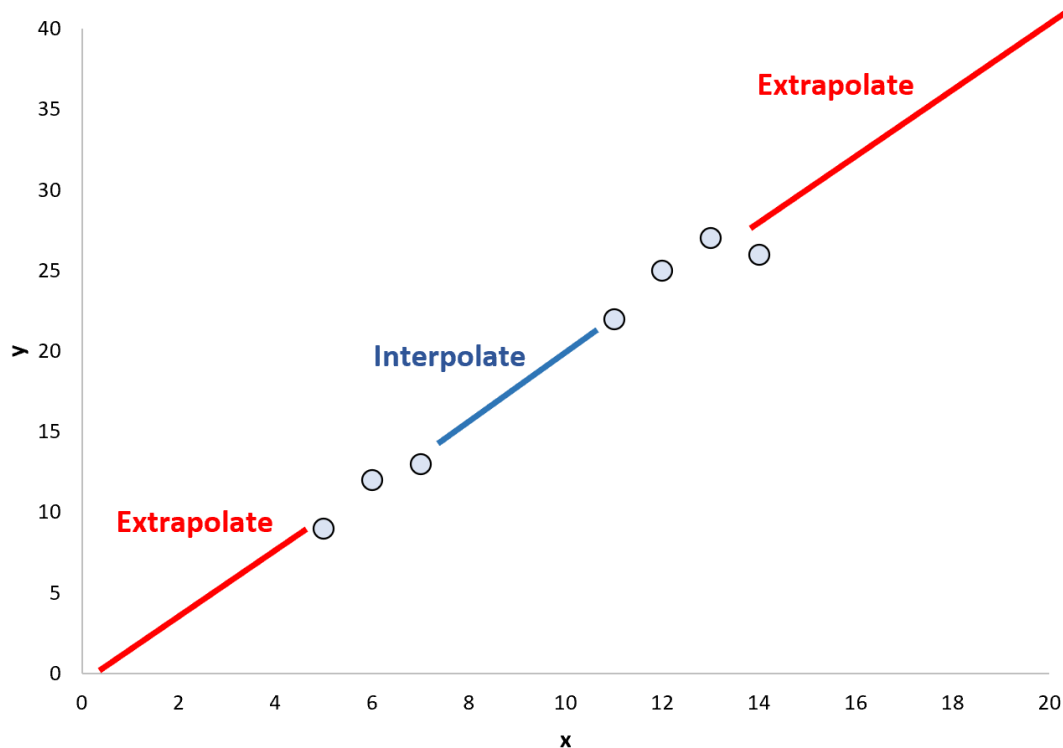
Figure 5: Difference between the interpolation (blue) and extrapolation (red) regimes. The former is reserved for inferences between known data points (blue dots) on the regression line, whereas the domain of the latter lies outside of it.
