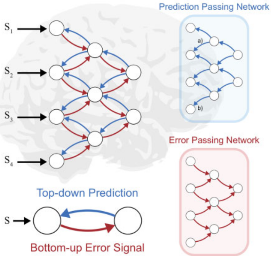
Figure 3: Top-down and bottom-up information transfer
